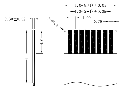
RECOMMENDED FPC/FFC DIMENSION
